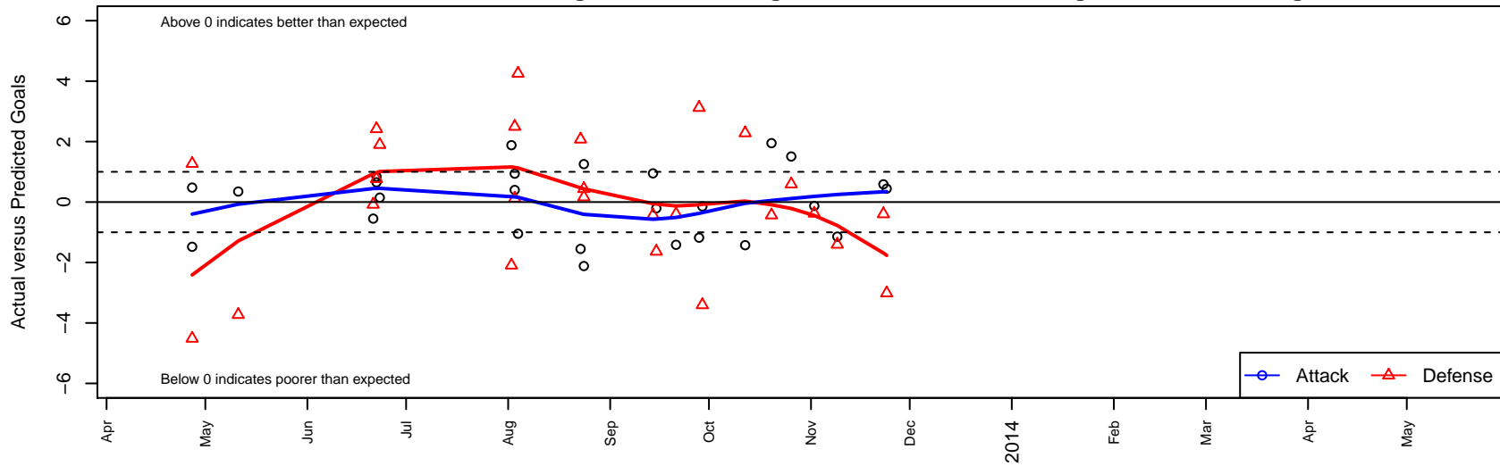
KVJSA Ellensburg FC Chargers B99 Dots are actual minus expected GF (blue circles) and GA (red triangles). Blue line is smoothed change in attack strength. Red is smoothed change in defense strength.
